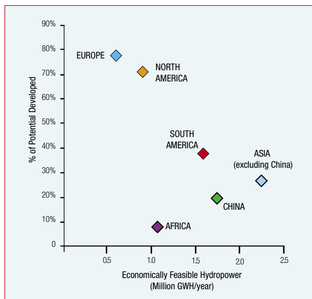
Figure 4.1 Hydropower Development
