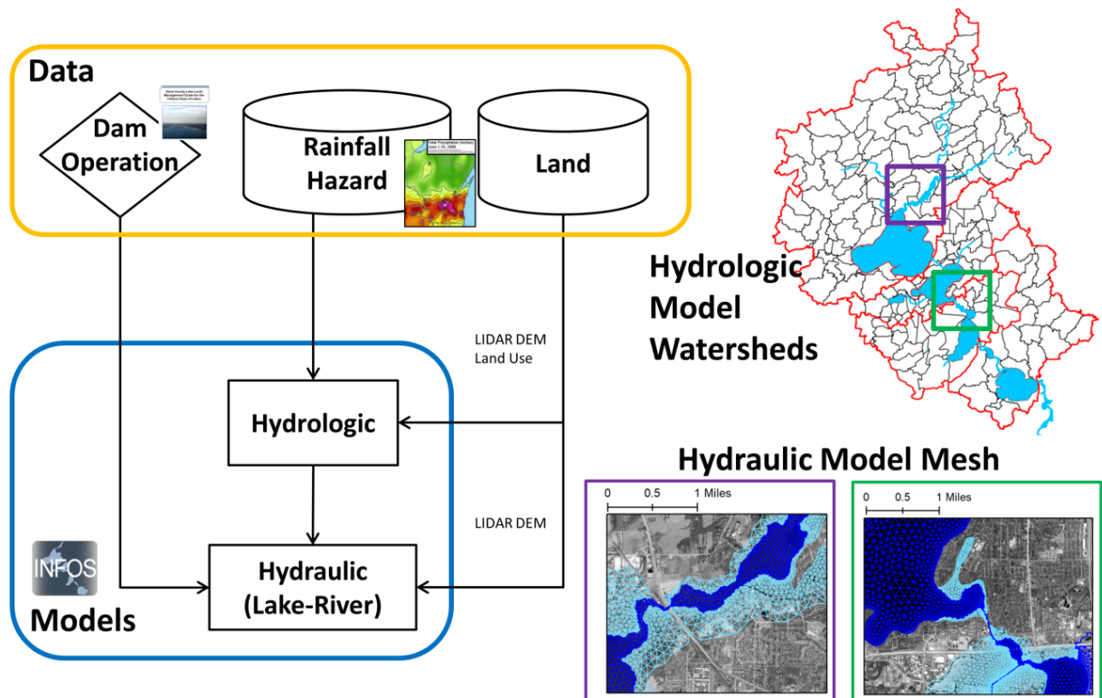
Figure 6: Modeling Framework
