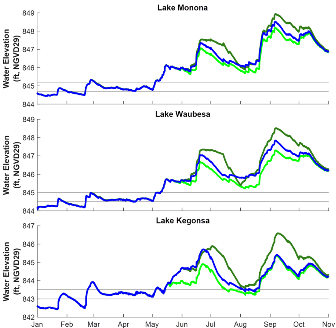
Figure 14: Aquatic plant management scenarios comparing dense aquatic plants (dark green), no aquatic plants (light green), and 2018 conditions (blue).
