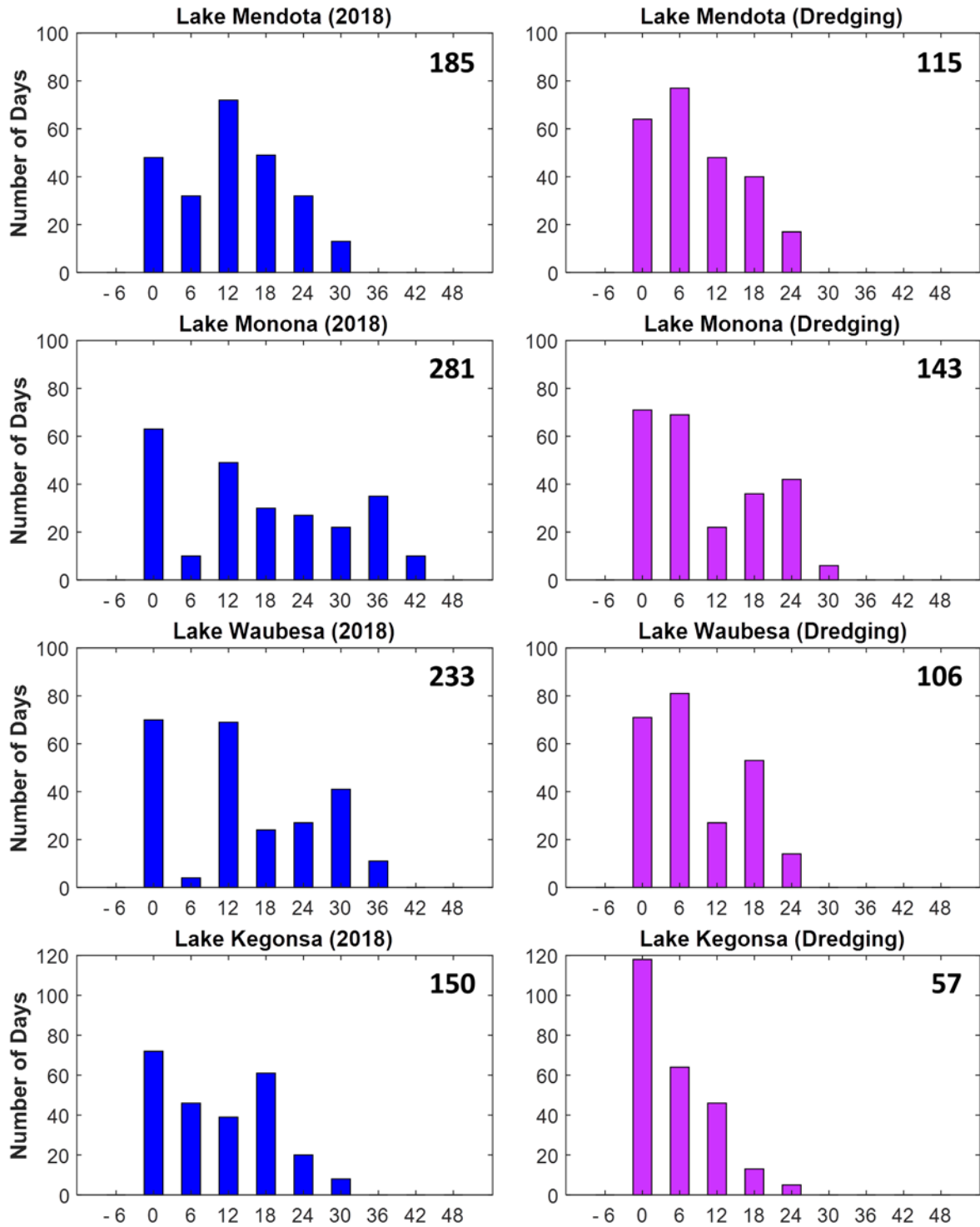
Figure 26: Number of days within water level ranges comparing 2018 levels on the left (blue bars) to dredging the Yahara River (purple bars). The x-axis shows the summer minimum/maximum water level range as denoted by 0 and each six inch increment above or below the summer range (x-axis).
