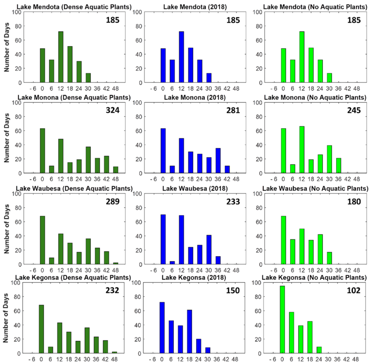
Figure 15: Number of days within water level ranges comparing dense aquatic plants on the left (dark green bars), 2018 in the center (blue bars), and no aquatic plants on right (light green). The x-axis shows the summer minimum/maximum water level range as denoted by 0 and each six inch increment above or below the summer range (x-axis).
