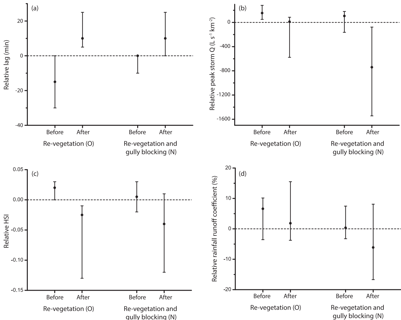
Fig. 5. Median relative differences between the treatment and control sites for the largest 10 storms before and after restoration: (a) lag time, (b) peak discharge, (c) Hydrograph Shape Index, and (d) percent runoff. Positive values indicate that the metric is greater at the treatment site than at the bare control, while negative values indicate the opposite. Error bars represent the interquartile range.
