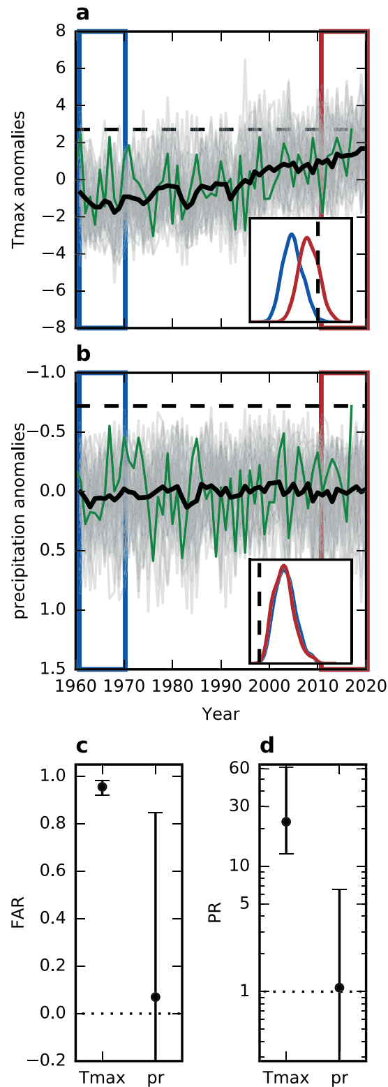
Figure 2. Time series of July–August (a) mean daily maximum temperature (Tmax, °C) and (b) mean daily precipitation (pr) anomalies. Precipitation is plotted as relative anomalies on an inverse scale. Observations are shown in green, and bias-corrected CanRCM4 realizations are in gray with the ensemble mean in bold black. Dashed lines (in a and b) mark the observed 2017 values. Anomalies (relative to 1981–2010) are expressed as differences for Tmax and ratios for precipitation, centered on 0. Probability density curves (insets) are from the CanRCM4 ensemble from decades outlined in corresponding colors. The fraction of attributable risk (FAR; c) and probability ratio (PR; d, log scale) for observed 2017 anomalies are plotted with 90% confidence intervals.
