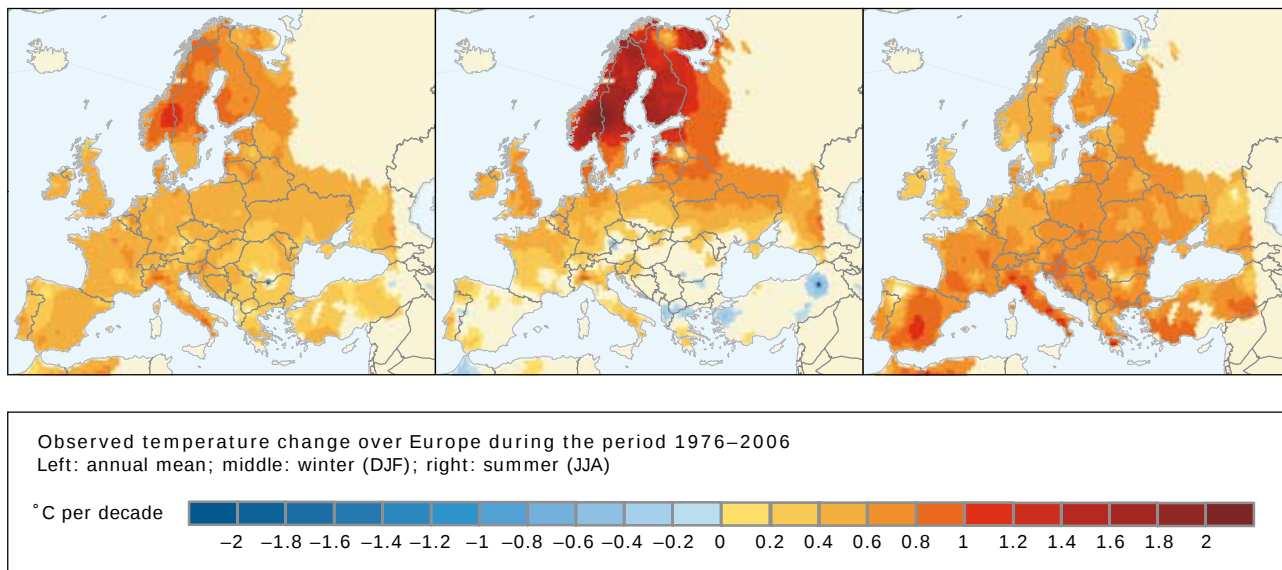
Map 5.1 Observed temperature change over Europe 1976–2006
