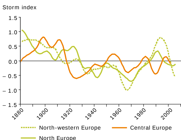
Figure 5.7 Storm index for various parts of Europe 1881–2005
