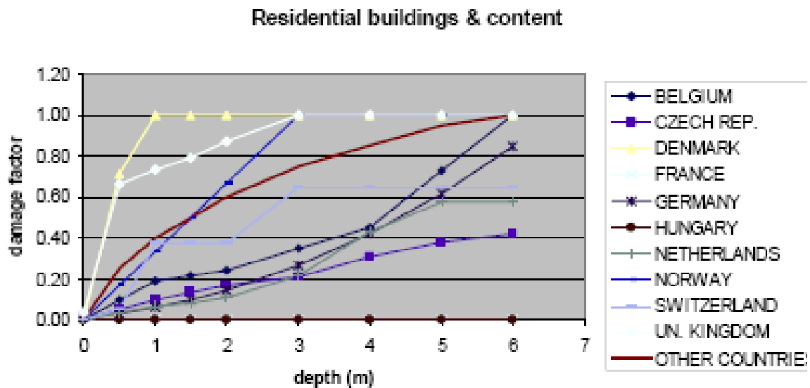
Figure 2: Damage factor for residential buildings including inventory (from Barredo 24 )
