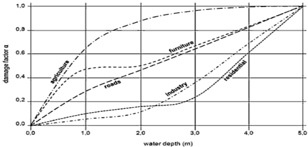
Figure 14: Example of absolute and relative depth damage functions
