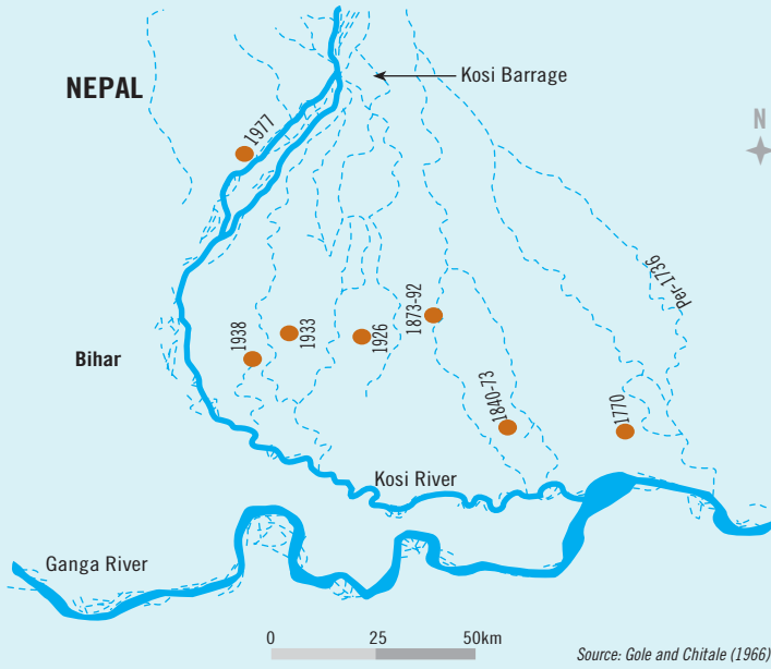
Figure 2.3: Koshi embankment breach
