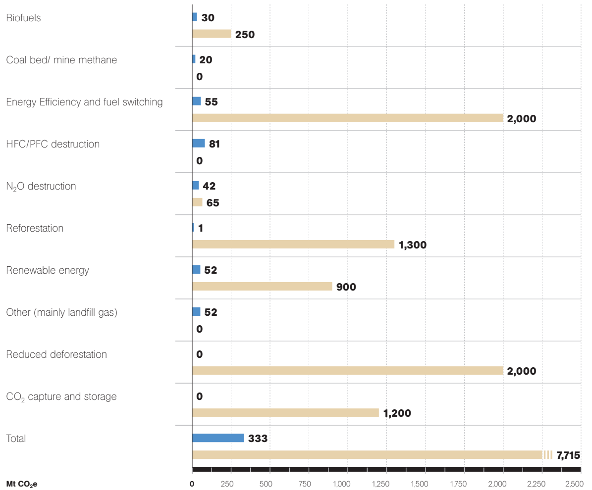
Figure VII-39. Estimated carbon market size for high demand estimate
