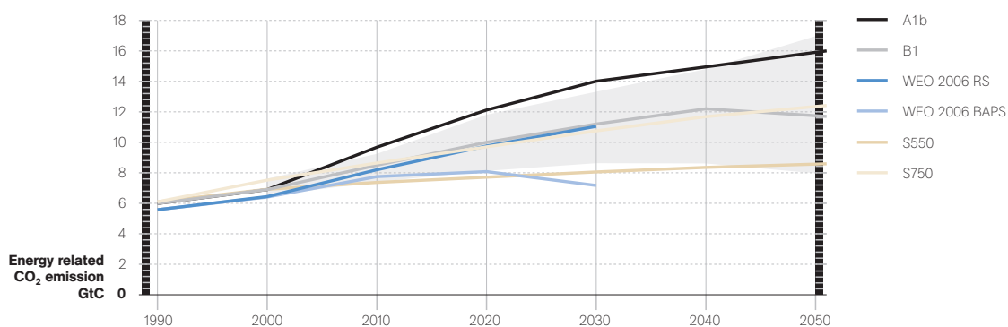
Figure II-3. Emissions projections of the scenarios used for the analyses and the scenario literature
