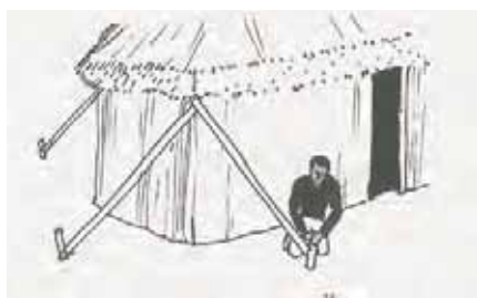
Lateral bracing
