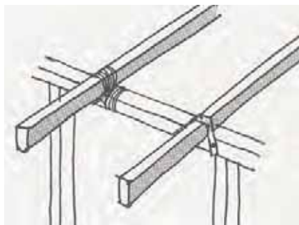
Tying techniques
