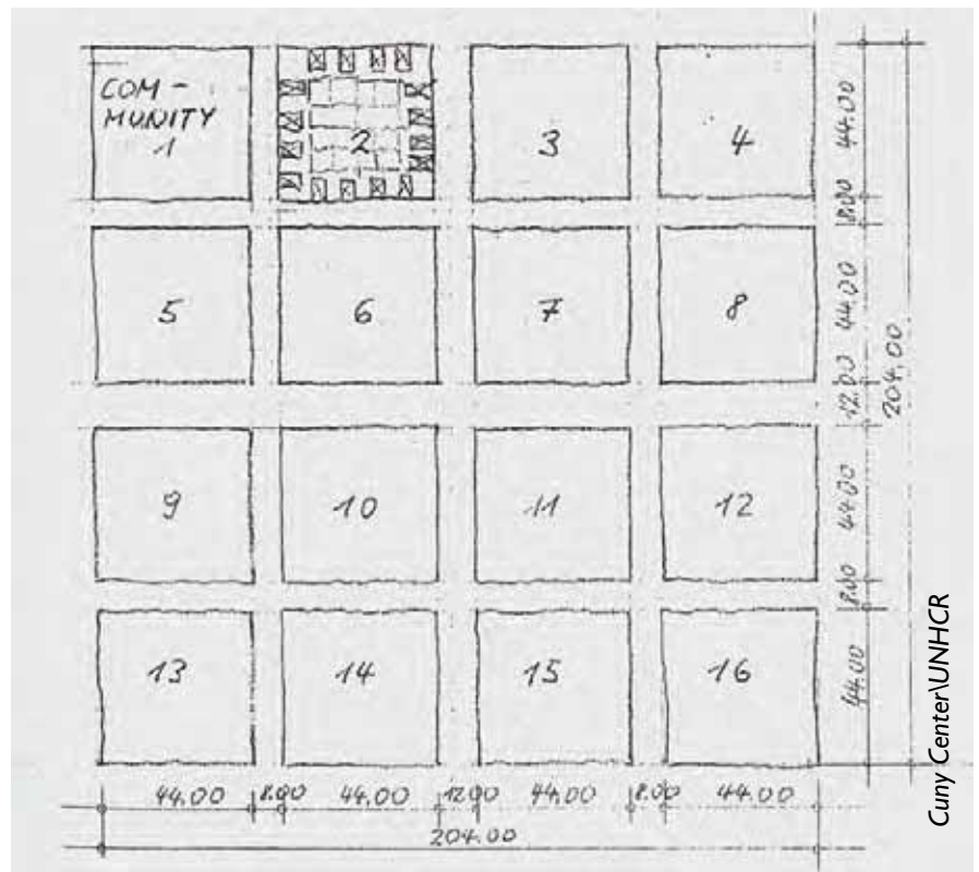
Sector plan
