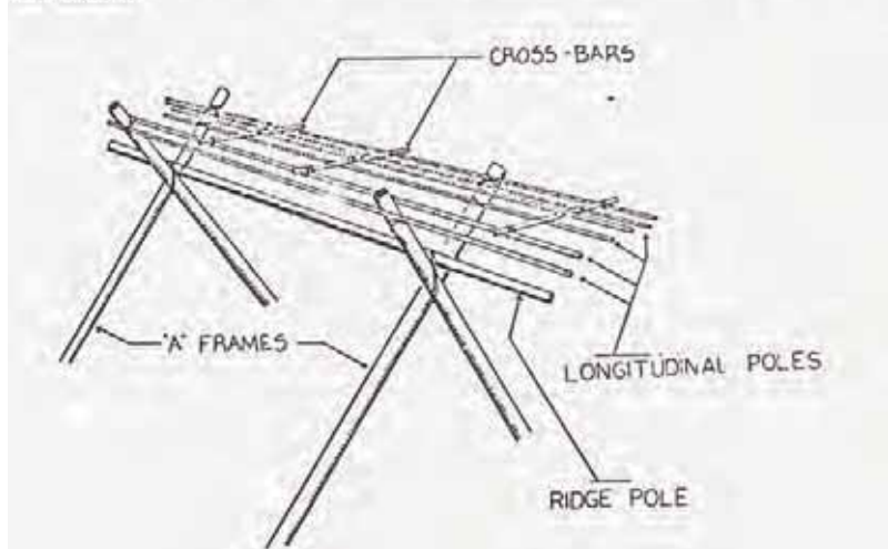
Shelter design details
